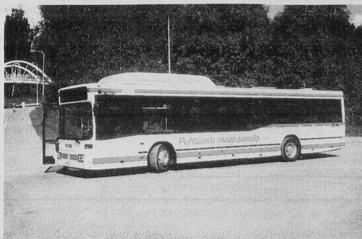
The supply of natural gas is on the roof of the bus.
