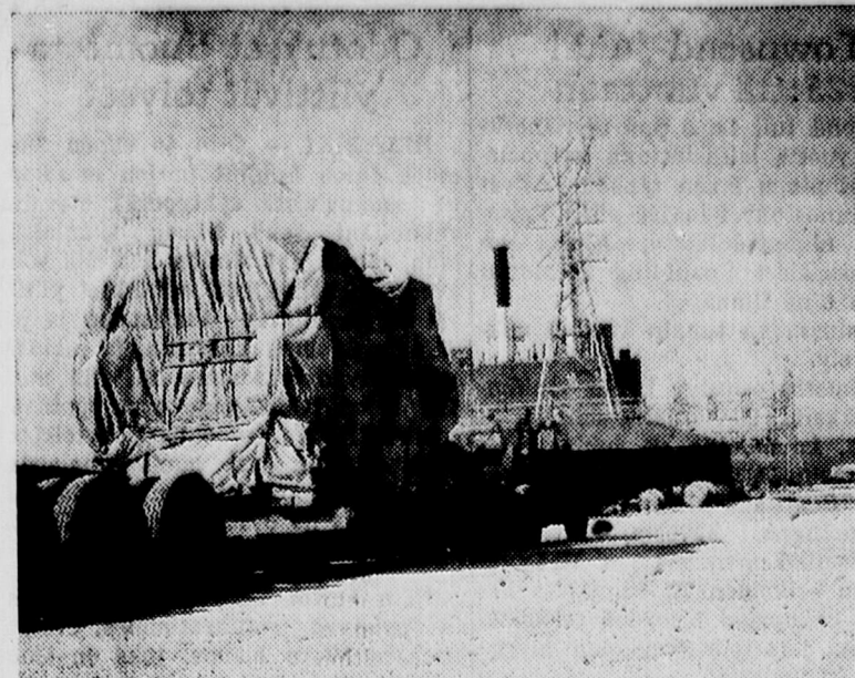
The stator for Central Maine Power Company's second 44,000-kilowatt generator arrives at Yarmouth Station on Cousins Island. This and its companion unit which is already in place are by far the largest units for generating electric power yet installed. Unit 1 is scheduled to start supplying power to electricity users in December. Unit 2 will go on the line next year.
