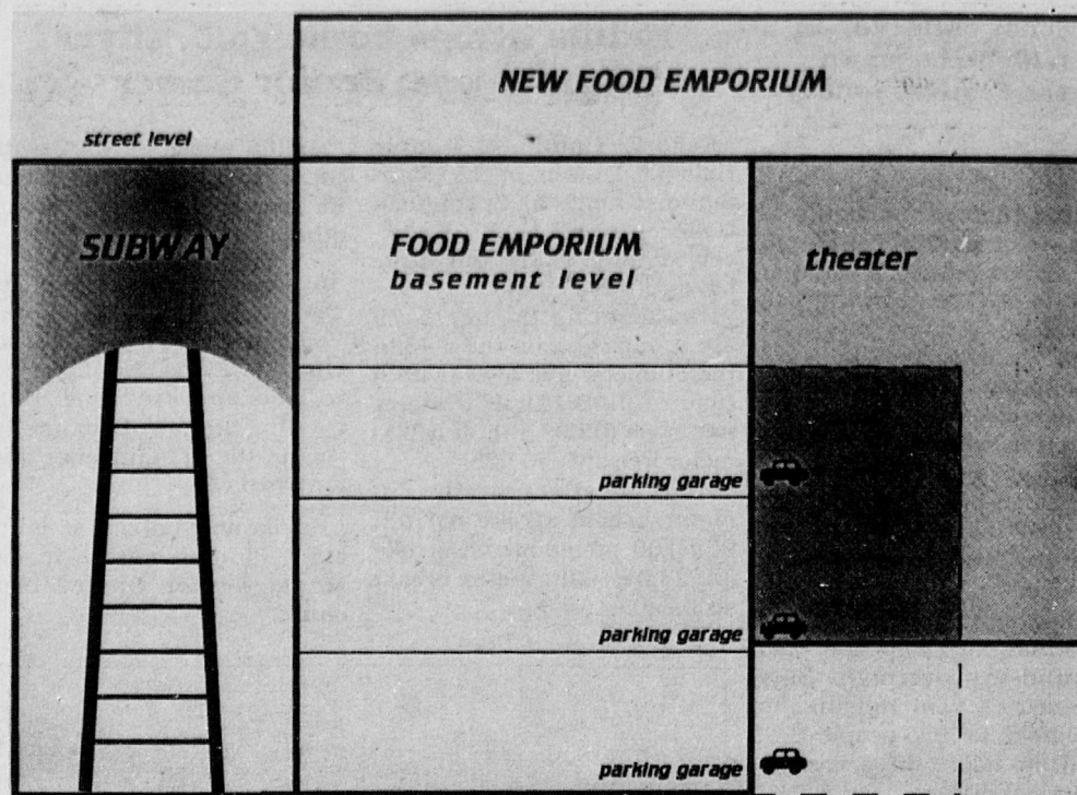
Cross section showing the sensitive and complex array of facilities beneath and surrounding the new Food Emporium, 10 Union Square, Manhattan (NY), that Nurminen Construction had to deal with during renovation of the space. Nurminen Construction drawing
