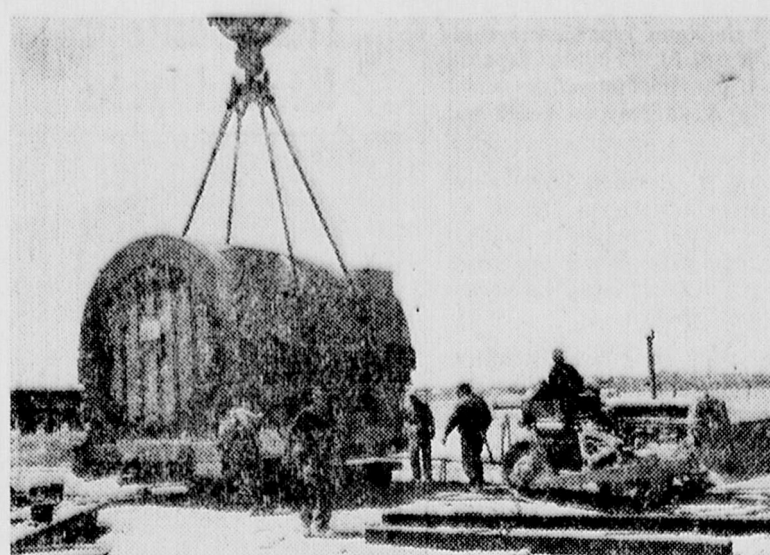
A bull-dozer swings the 103½-ton stator of Central Maine Power Company's first generator scheduled for installation at Yarmouth Station. The stator had just been picked off a drop-center railroad car at Portland by a powerful, steam-operated, stiff-leg derrick.
